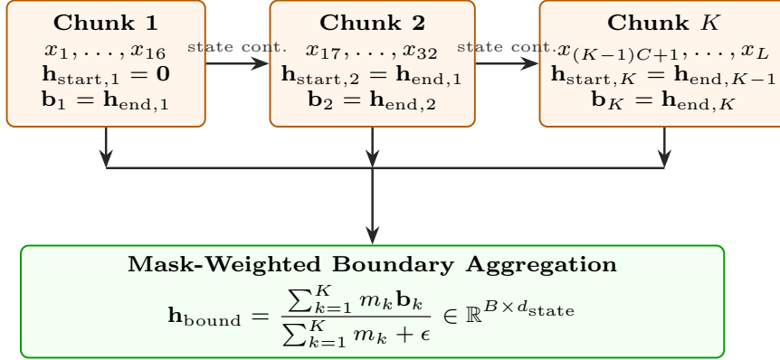
Fig. 2 State-continuous chunk-wise recurrence with boundary state extraction. Hidden states propagate across chunk boundaries without resets, and mask-weighted aggregation prevents padding bias.
